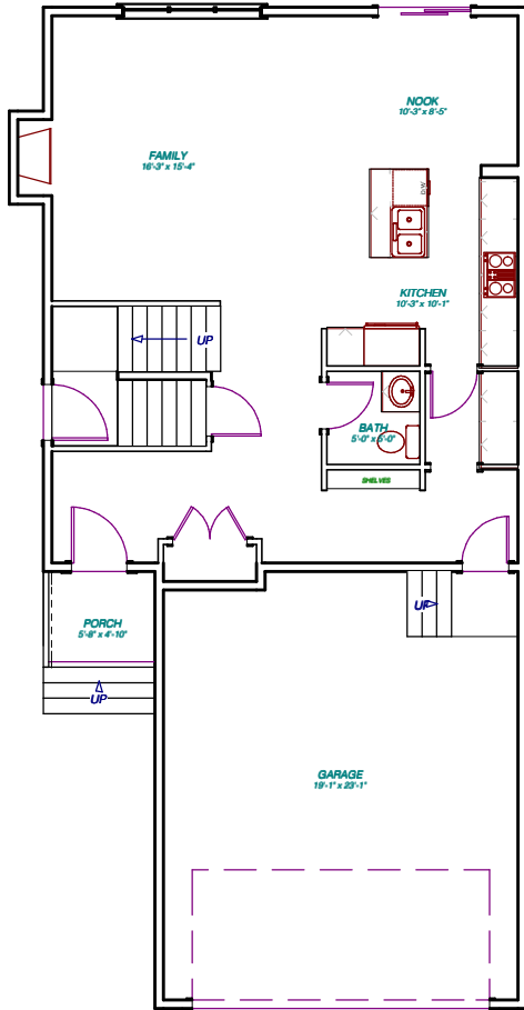
MAIN FLOOR : 825 SQ.FT.
