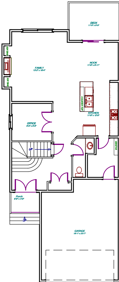
MAIN FLOOR : 949 SQ.FT.
